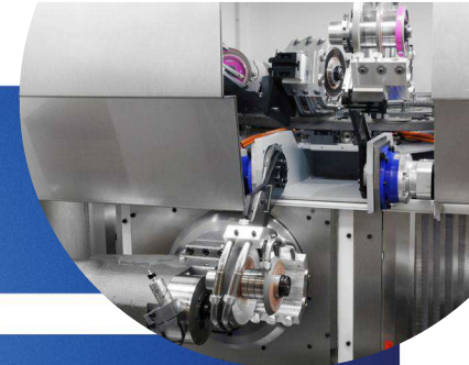
Ultra-compact 15-position wheel/nozzle changer - wheel pack and nozzle change under 11 seconds - tool unload/load simultaneously during wheel change - lean manufacturing - no additional footprint
